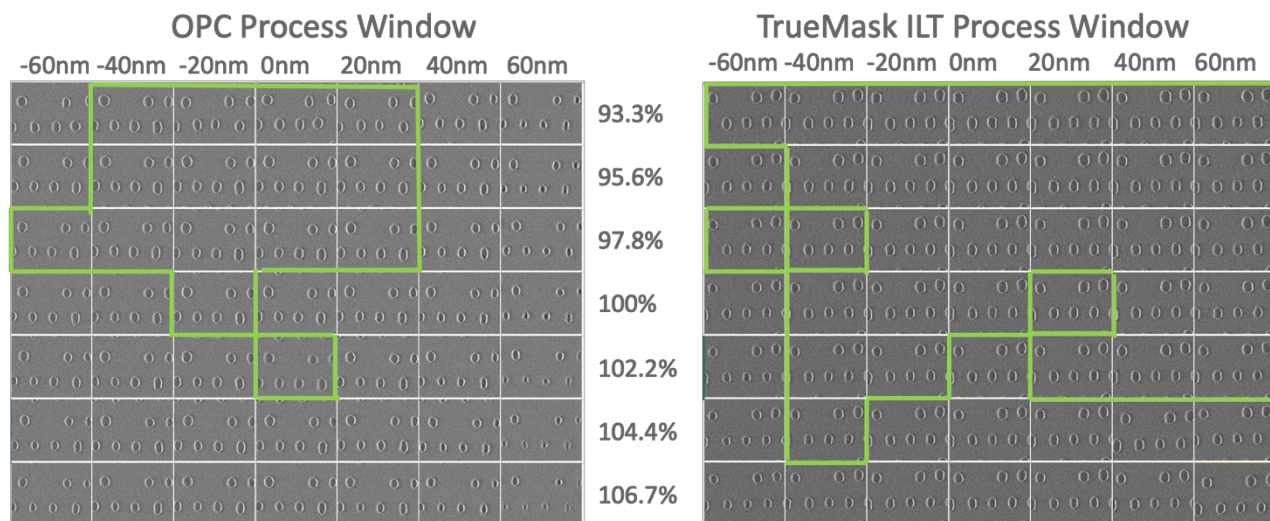
Figure 20: Wafer print matrix for a cut layer type of design. Highlighted regions are within process window
