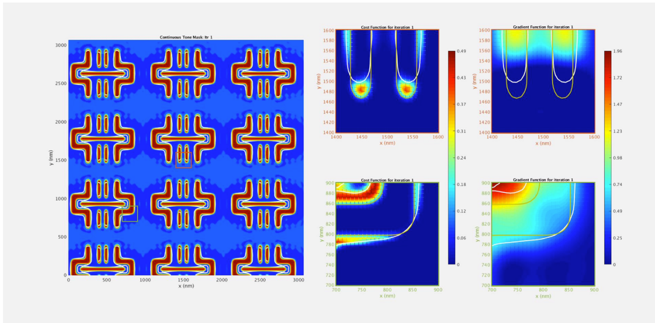
Figure 12: Mask pattern, simulated wafer contour and its target, cost function and cost gradient at the beginning of the TrueMask ILT optimization
