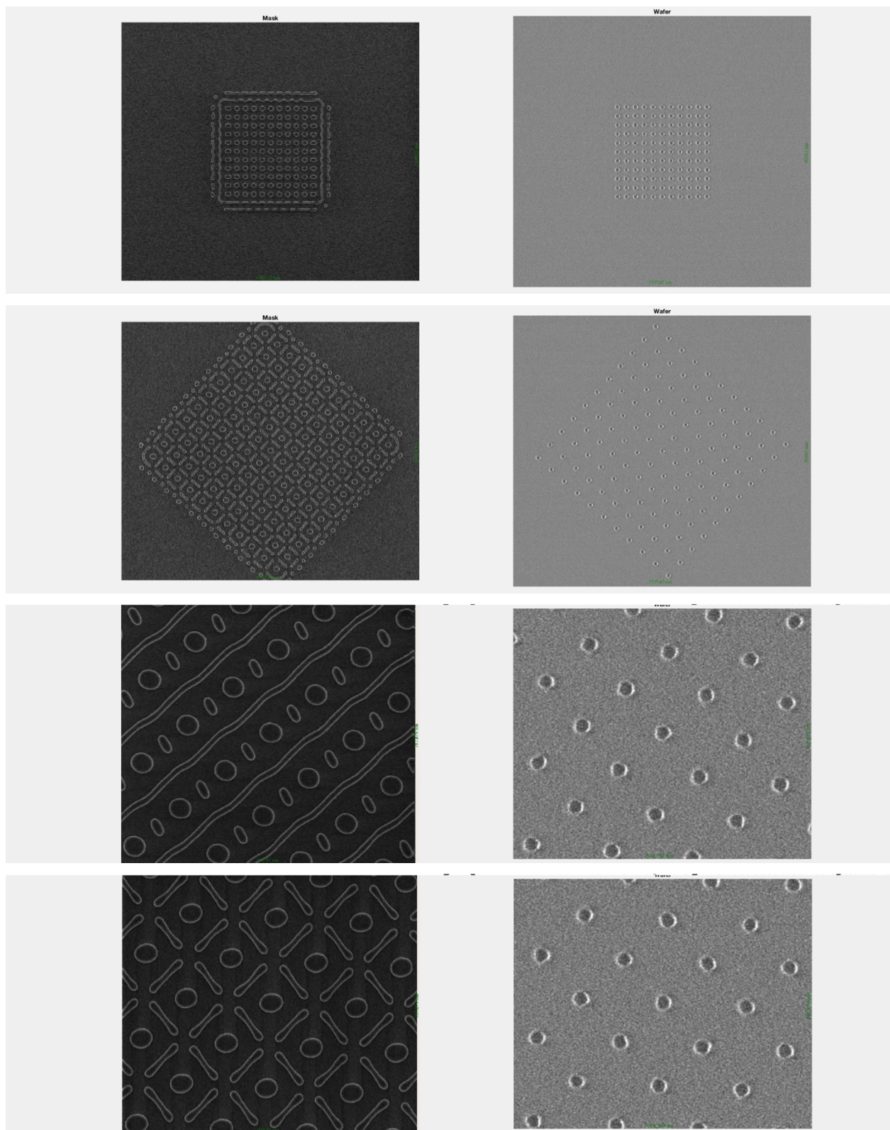
Figure 18: In each pair, the ones on the left are TrueMask ILT curvilinear mask written by NuFlare multi-beam mask writer for different pitches & orientations, the ones on the right are corresponding wafer print using Micron process
