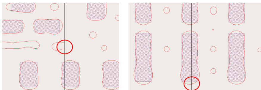
Figure 7: Stitching errors occur when a chip is partitioned for parallel computing and re-assembled
