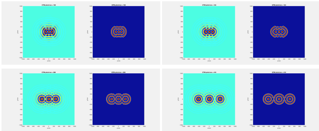
Figure 14: Continues Tone Mask (CTM) and Final ILT mask for three contacts in symmetric position at different pitches showing TrueMask ILT solutions are continuous and symmetric
