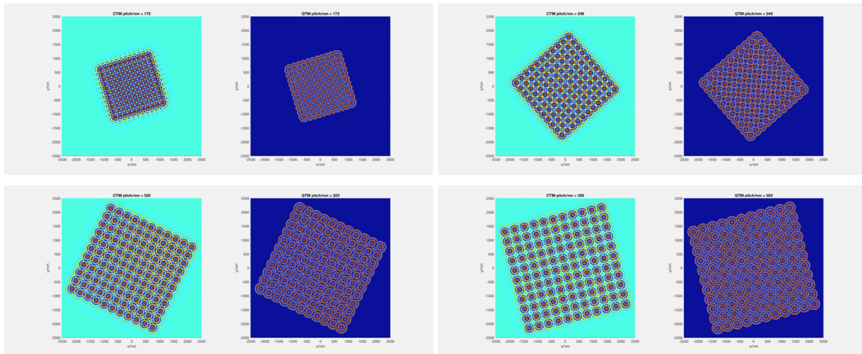
Figure 16: CTM and Final ILT mask for an equal pitch contact array at on-grid and off-grid situation, pitch change, plus rotation demonstrating TrueMask ILT solutions are symmetric and rotation invariance
