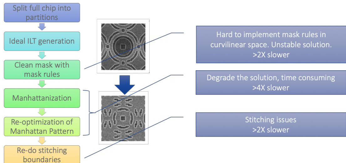
Figure 5: In the conventional ILT flow, in order to generate a solution for full chip and for VSB mask writer to write, the run time has increased order of magnitude due to all these extra steps
