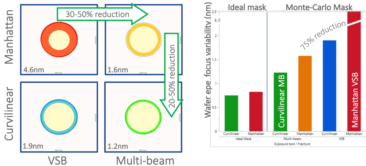
Figure 4: Study[20] shows the mask variation PV bands can be reduced 75% by switching from writing Manhattan pattern on VSB mask writer to writing curvilinear mask pattern on multi-beam mask writer
