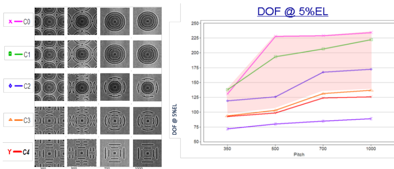
Figure 2: Study of different complexities of ILT mask patterns and their corresponding process window shows unconstrained curvilinear ILT mask patterns produce the largest process window [18]
