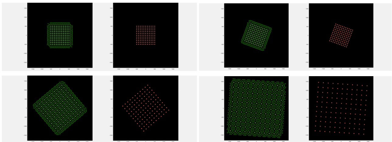
Figure 17: In each pair, the ones on the left are TrueMask ILT curvilinear mask designs for different pitches & orientations, the ones on the right are corresponding wafer target & simulated wafer contours
