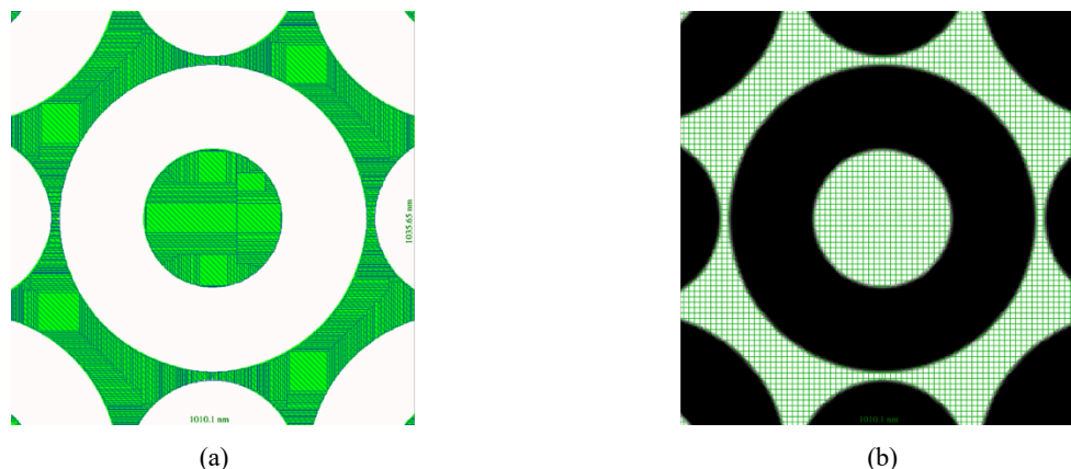
Figure 3: (a). Conventional VSB mask writer: generates too many shots, takes too long to write; (b). Multi-beam mask writer: designed for curvilinear ILT, writes any shape in constant time[20]
