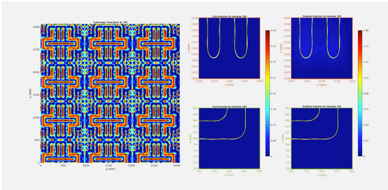
Figure 13: Mask pattern, simulated wafer contour and its target, cost function and cost gradient at the end of the TrueMask ILT optimization
