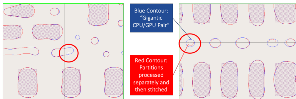
Figure 9: No stitching errors occurs in TrueMask ILT
