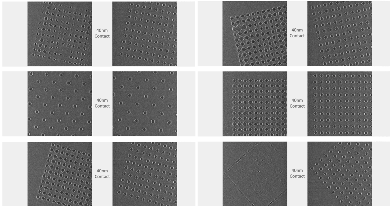
Figure 19: In each pair, the ones on the left are OPC wafer printed by Micron process at different process conditions, the ones on the right are TrueMask ILT wafer printed at the same process condition
