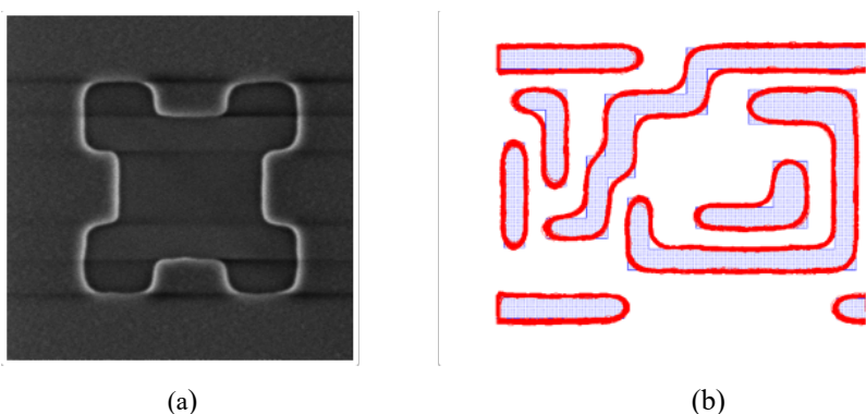
Figure 10: All shapes on masks and wafers are curvilinear, even if the input geometries are rectilinear: (a) Manhattan OPC mask pattern with serif shows curvilinear nature on mask; (b). Wafer pattern designed as Manhattan shows curvilinear nature from simulation
