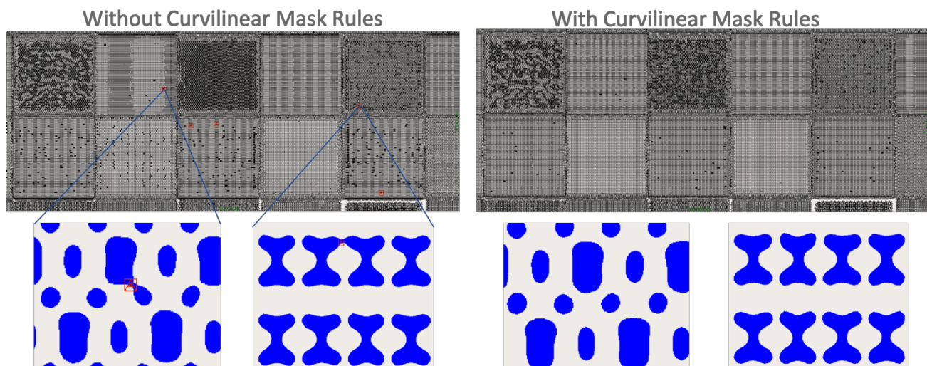
Figure 11: Comparison of TrueMask ILT without and with integrated MRC. The top row shows the layout where the red marks are MRC violations detected by D2S mask verification
