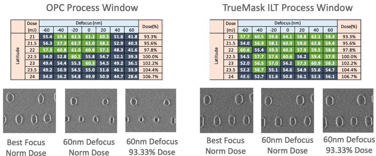
Figure 21: Process window CD measurements. The highlighted regions are within process window
