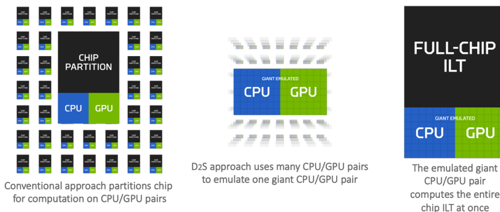
Figure 8: TrueMask ILT, although comprising many GPU/CPU pairs, has been holistically designed so that it behaves as a single GPU/CPU pair, iterating on the entire chip as a whole, and avoiding stitching errors
